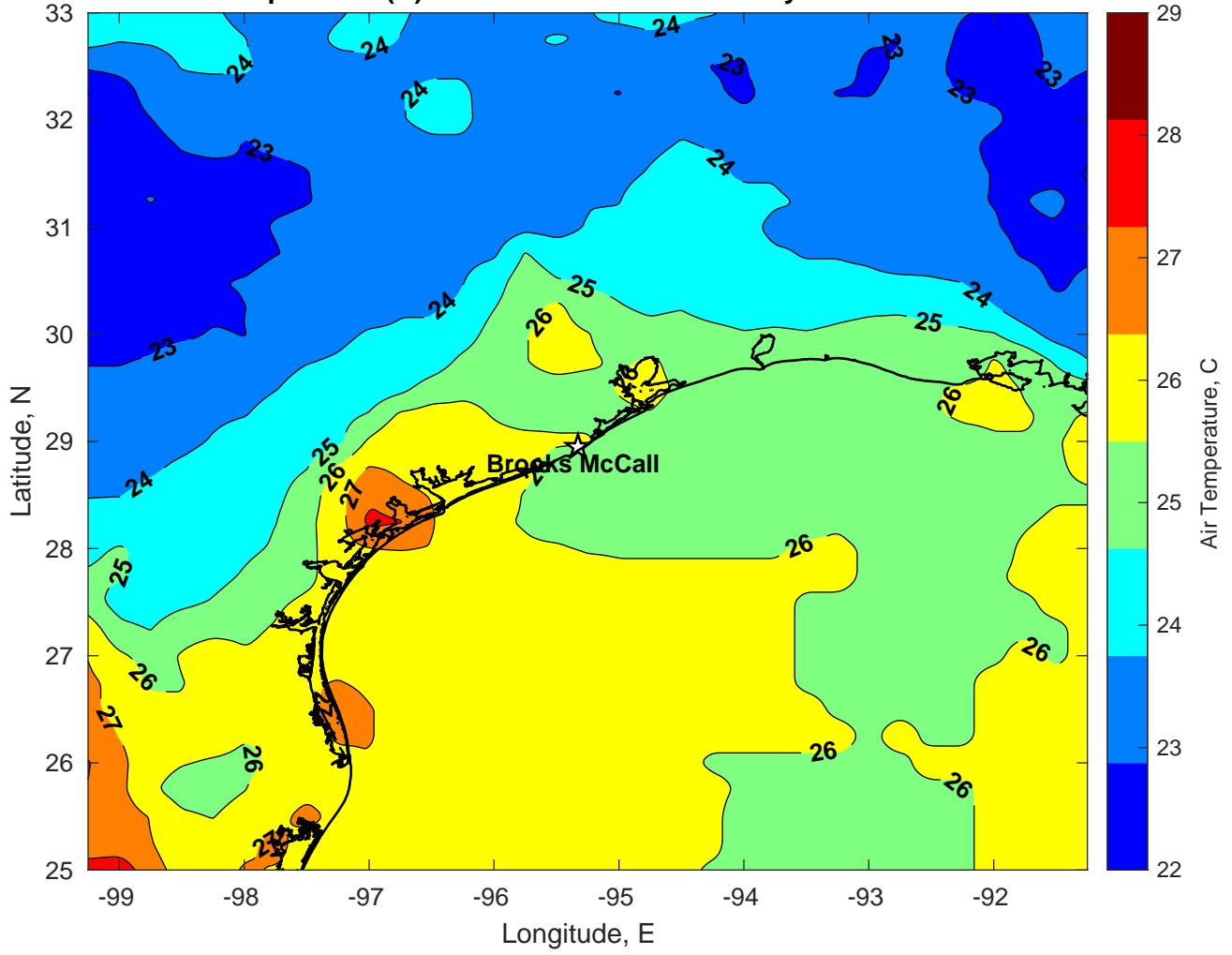
Air Temperature (C) for Brooks McCall at 07-May-2024
